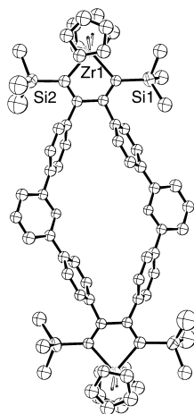
Figure 3. ORTEP depiction of the solid-state molecular structure of 18 .
