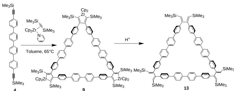
Scheme 4. Coupling of diyne 4 by an alternative [\text{Zr}^{\text{II}}(\text{Cp})_2] reagent and preparation of 13 .
