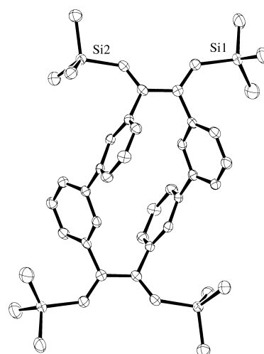
Figure 2. ORTEP depiction of the solid-state molecular structure of 20 .
