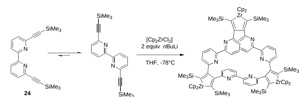
Scheme 5. Cyclotrimerization with diyne 24 .
