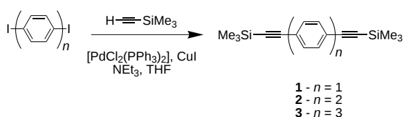
Scheme 1. Synthesis of diynes 1–3 by the general Pd-catalyzed coupling route.
