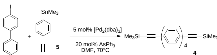
Scheme 2. The preparation of tetraphenylene diyne 4 .
