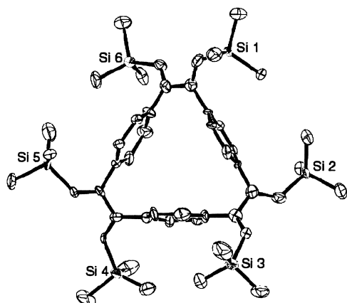
Figure 1. ORTEP depiction of the solid-state molecular structure of 10 .
