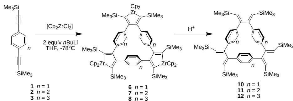
Scheme 3. Use of diynes 1–3 for the preparation of 10–12 .
